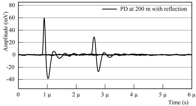
Fig. 8. PD fault location 200 m from the PD detector with reflection from far end on a 500 m cable.
