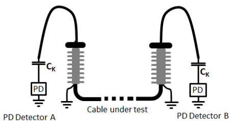
Fig. 12. Measurement setup for double sided measurement with PD detector A on the left side and PD detector B on the right side.
