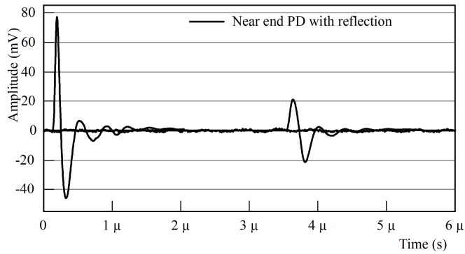
Fig. 7. Near end PD fault location with reflection from far end on a 500 m cable.
