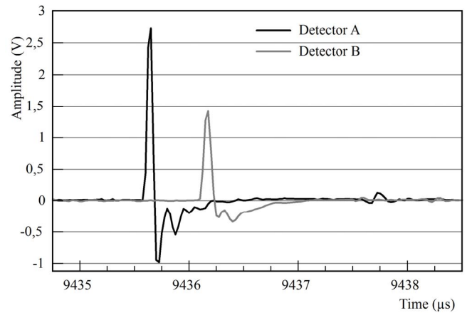
Fig. 13. Double sided measurement on a 644 m long medium voltage cable.
