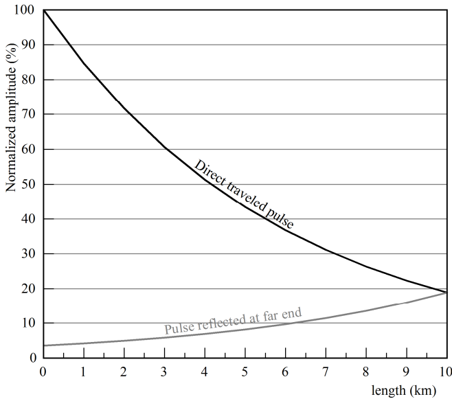
Fig. 5 Normalized PD amplitude attenuation on both sides of a 10 km long cable for double sided measurement (black). The reflection for the single sided measurement is the grey curve.
