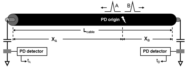
Fig. 4. Setup for the double sided PD measurement with fault localization functionality. t_A and t_B are the times were the direct travelled partial discharge waves are measured. Both PD detectors have to be synchronized for PD origin localization.
