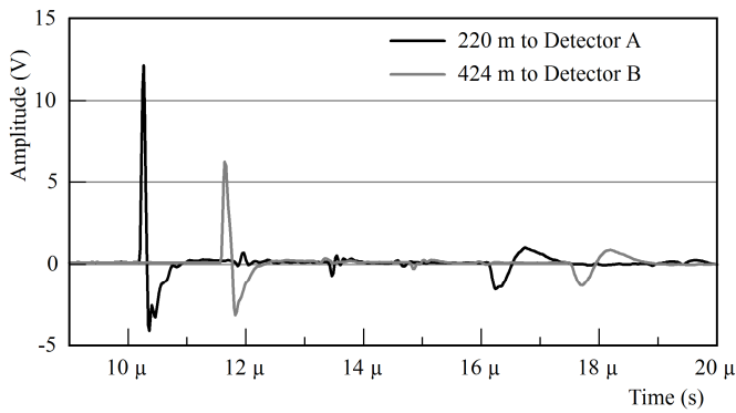
Fig. 11. Double sided PD measurement data with PD origin at 220 m from Detector A and 424 m from Detector B.
