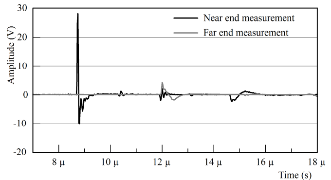
Fig. 10. Double sided PD measurement data. Detector A is located at the near end side of the cable and Detector B on the opposite far end side. The PD pulses are injected at the near end close to Detector A.
