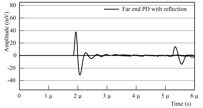
Fig. 9. PD fault location at the far end from PD detector and reflection over near and far end.
