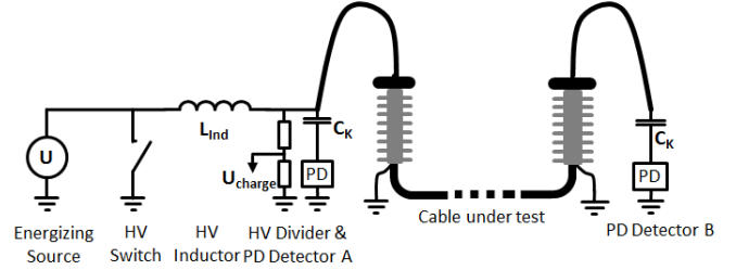
Fig. 3. Setup for two sided PD measurement with localization feasibility. DAC excitation circuit and synchronized PD detector units.
