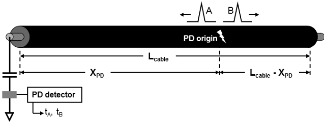
Fig. 2. Power cable with PD source emits two travelling waves A and B with speed v . The PD detector on the left side can calculate the PD origin with the aid of TDR analysis.
