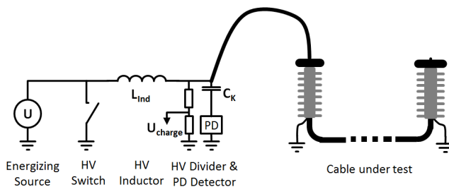
Fig. 1. Measurement setup for single sided PD measurement with DAC voltage excitation and PD detection circuit.
