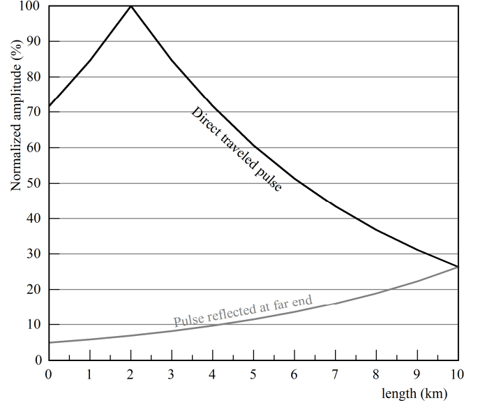
Fig. 6. Normalized PD amplitude attenuation with a fault location at 2 km seen from the left side. The reflection on the right side is colored in grey.
