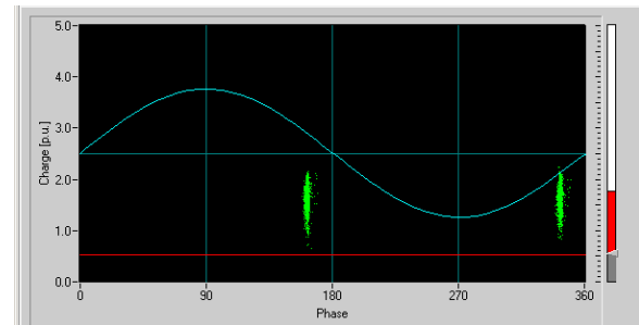
Fig. 8: Phase Resolved Partial Discharge pattern (PRPD) of the new UHF signal generator
