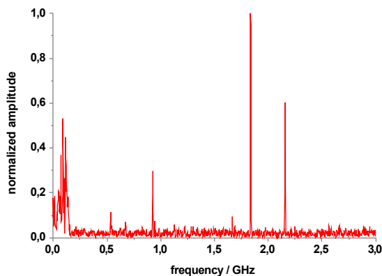
Fig. 12: Narrow-band disturbances during online measurement with 20 dB amplification
