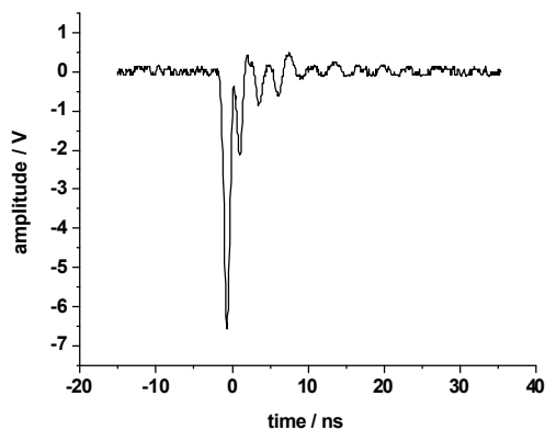
Fig. 5: Time signal of a UHF signal generator
